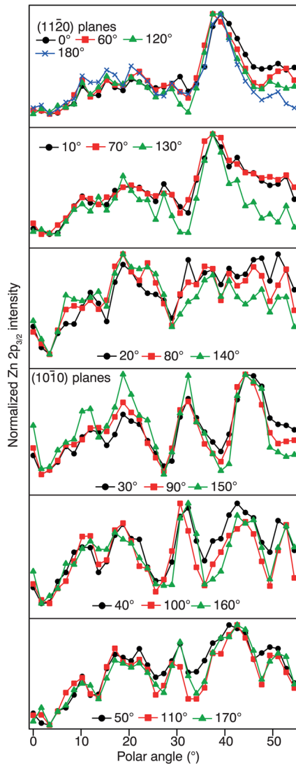
FIG. 3. (Color online) Polar angle ( \theta ) dependency of core-level peak intensities taken from the (0001) ZnO surface. Profiles were taken for each azimuthal angle ( \varphi ) in steps of 10^\circ and are grouped in \varphi intervals of 60^\circ to illustrate the sixfold nature of the measurement.
