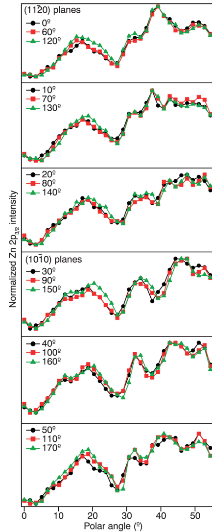
FIG. 4. (Color online) Polar angle ( \theta ) dependency of core-level peak intensity taken from the (000 \bar{1} ) ZnO surface. Profiles were taken every 10^\circ of azimuth ( \varphi ) and are grouped in \varphi intervals of 60^\circ to illustrate the sixfold nature of the measurement.
